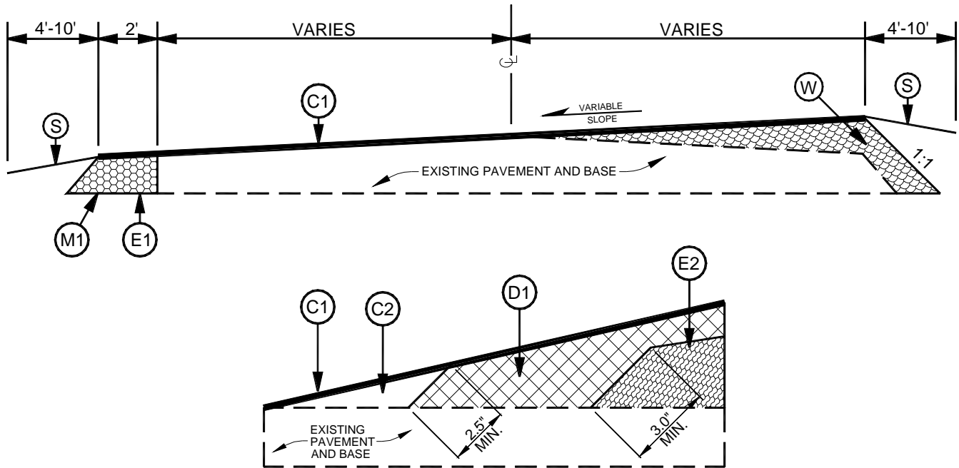
WEDGING DETAIL
